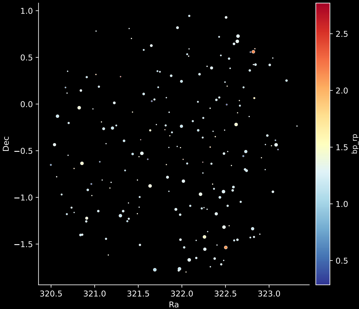
APOGEE DR17 Field: [353+50_btx] Stars: 201
