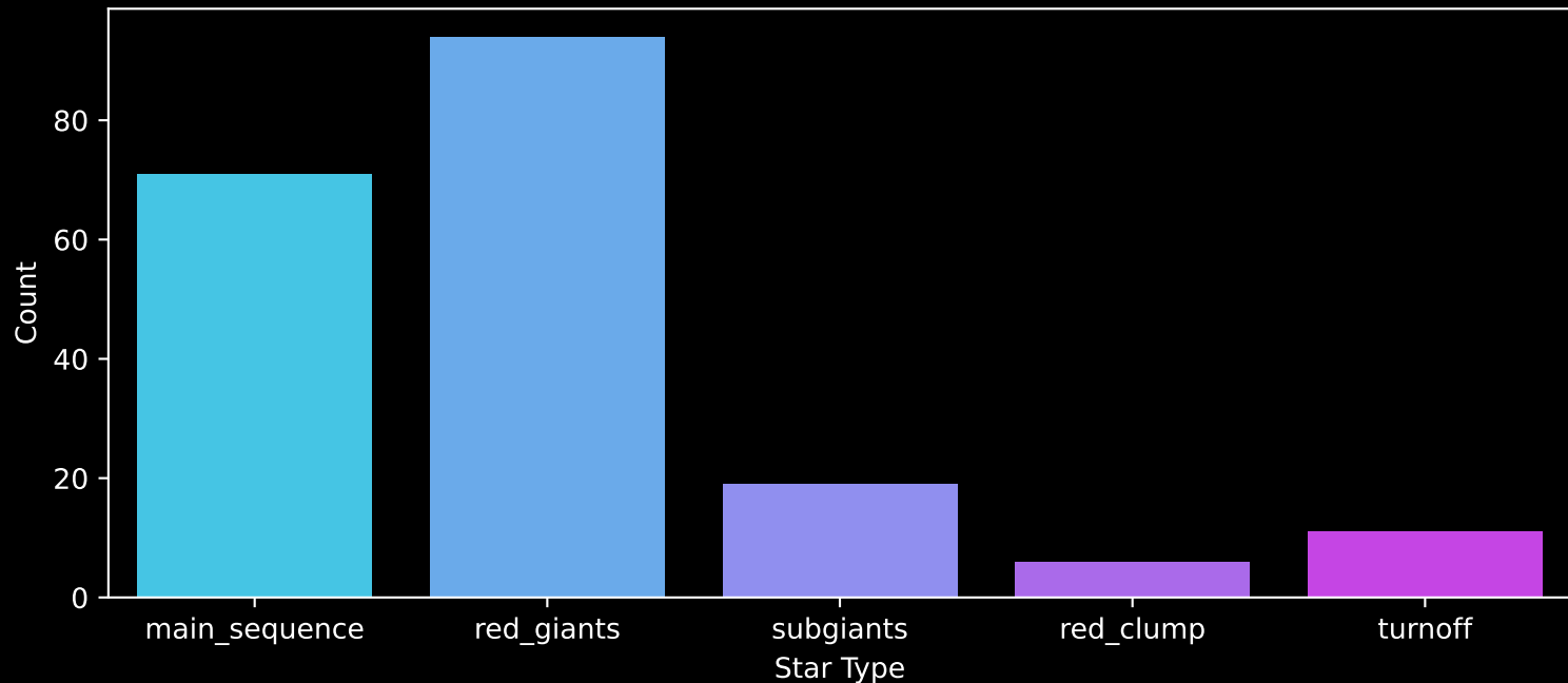
APOGEE DR17 Field: [353+50_btx] Count plot of Star Type
