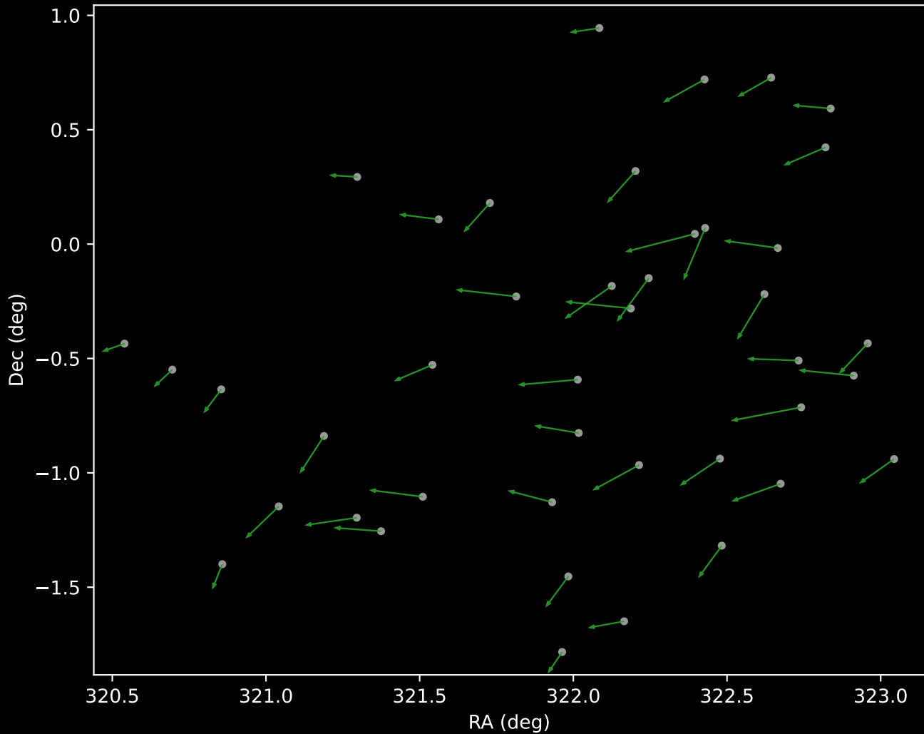
APOGEE DR17 Cluster 4 Proper Motion Vectors (n=42)
