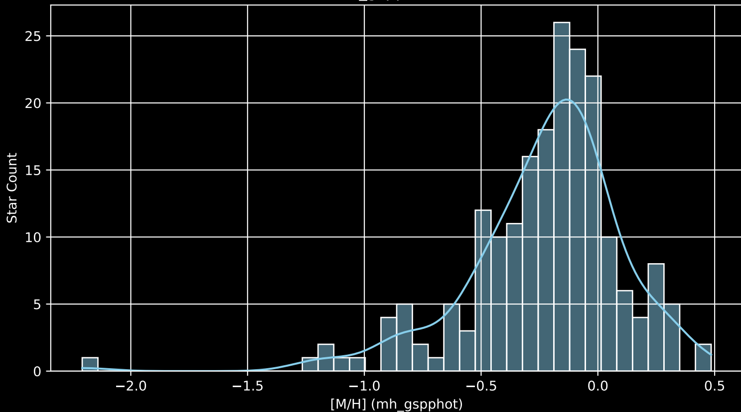
APOGEE DR17 Field: [353+50_btx [M/H] (mh_gspphot) (n= 200)
