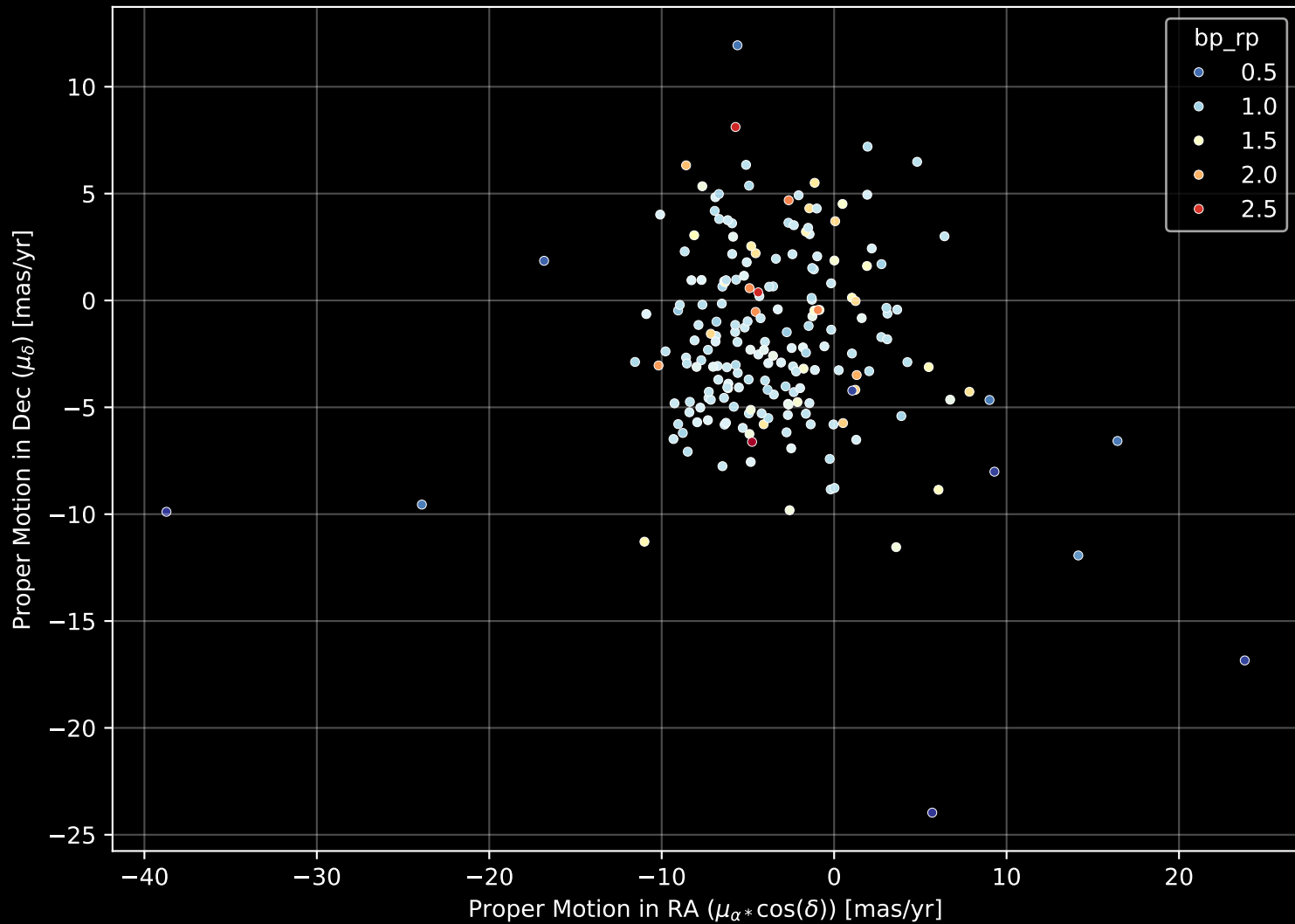
APOGEE DR17 Field: [353+50_btx] Proper Motion Diagram (n= 201)
