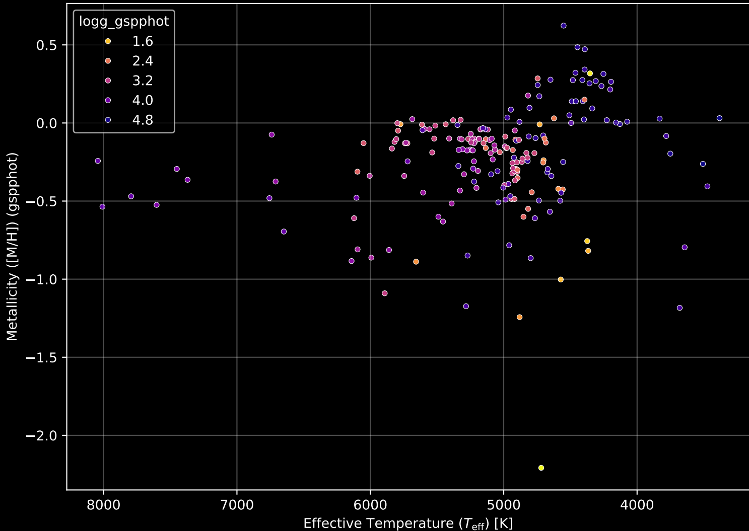
APOGEE DR17 Field: [353+50_btx] Stellar Population Parameters (n = 201)
