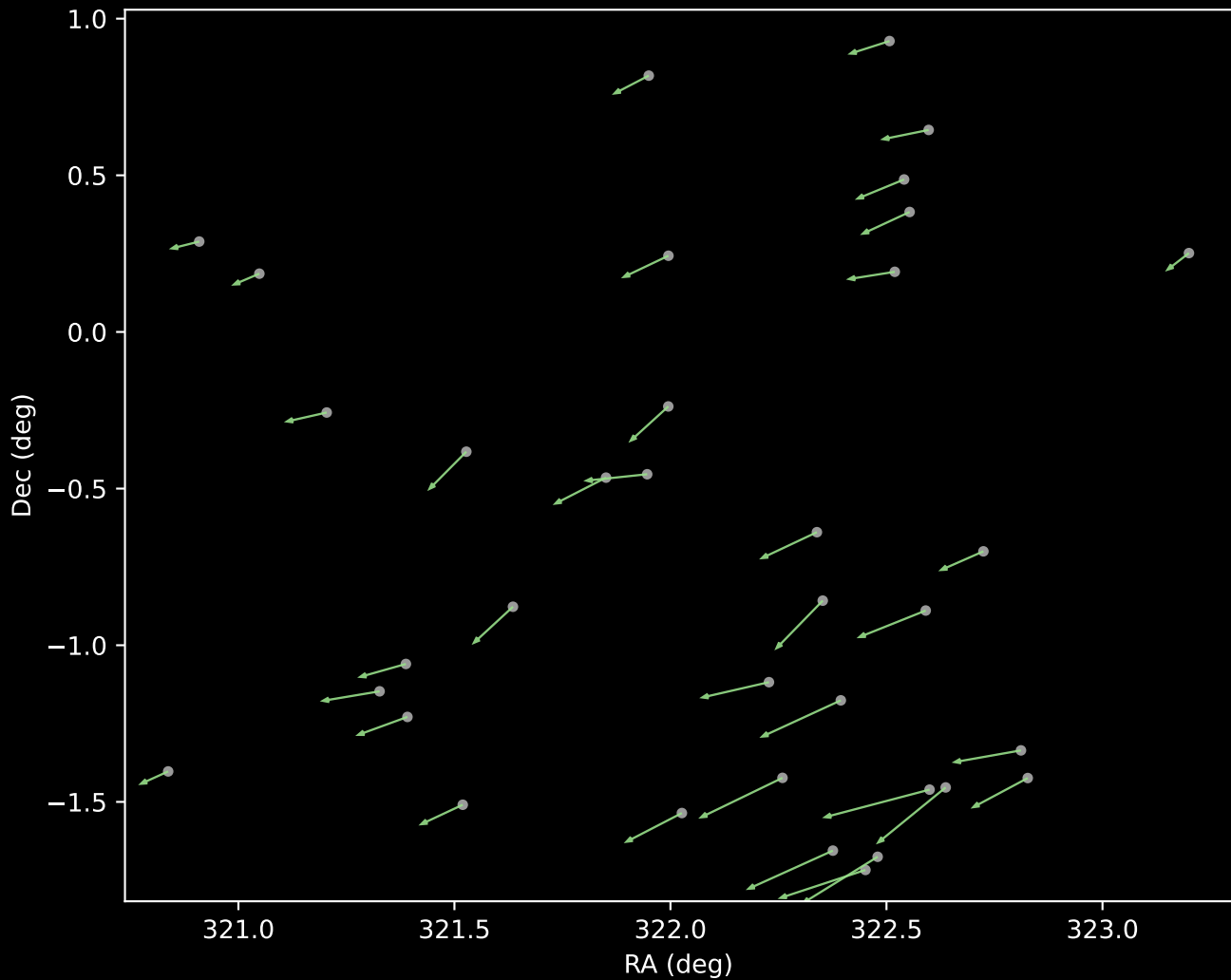
APOGEE DR17 Cluster 5 Proper Motion Vectors (n=36)
