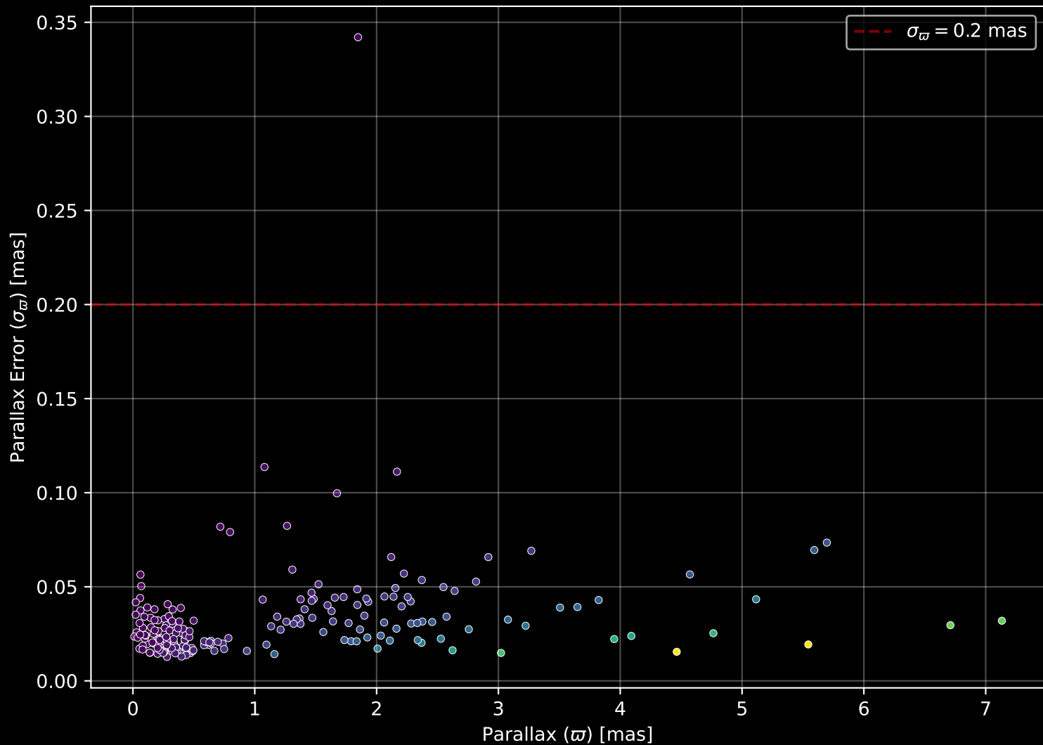
APOGEE DR17 Field: [353+50_btx] Parallax Quality (n= 201)
