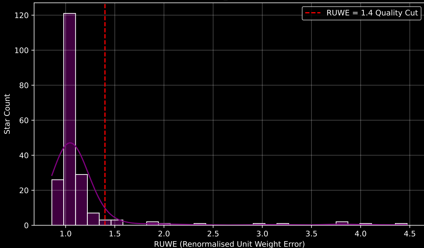
GAPOGEE DR17 Field [353+50_btx] RUWE Distribution (n= 199)
